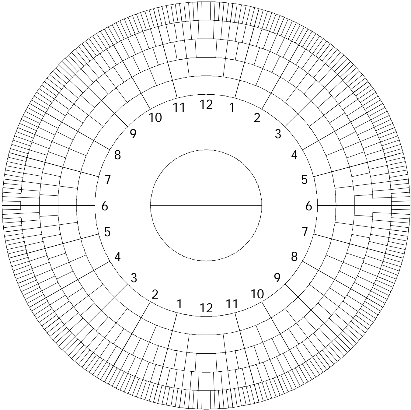
Equatorial Sundial Template 5-10-15-30-60 Minute Intervals
